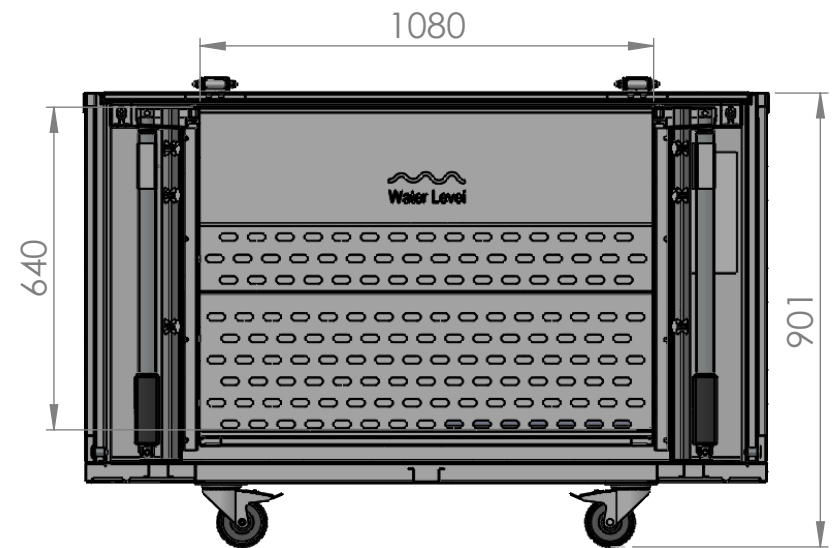
SECTION B-B
