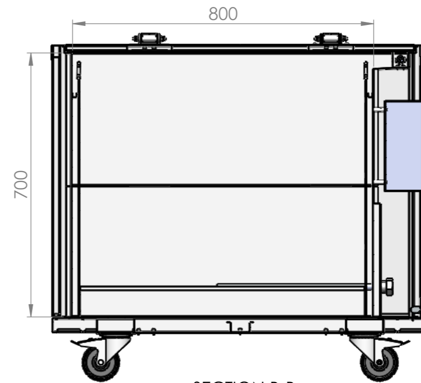
SECTION B-B
